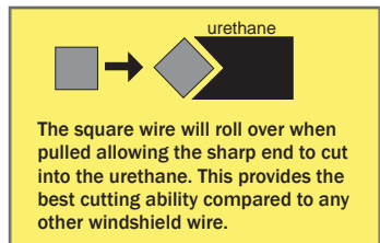
AIR WINDSHIELD REMOVAL KIT Pneumatic windshield knife with suction cups. Kit includes: windshield knife: 20,000 oscillations per minute, rear exhaust, teasing throttle and regulator provide easy speed control, flexible 12 position blade mount, includes 5 blades, suction cups: (2) 4 5/8" diameter double suction cups. Ratcheting tie down molded storage case. Stock No. 684
